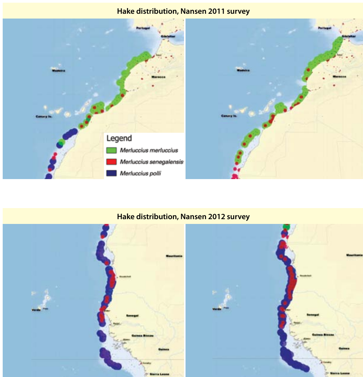
Figure 13: Hake distribution from R/V Dr Fridtjof Nansen surveys in 2011 and 2012.
