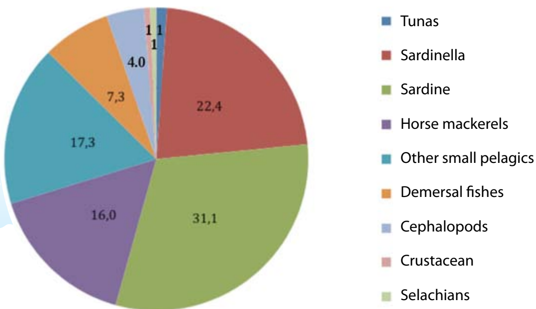
Figure 11: Average percentage of annual catches between 2000 and 2010 in the CCLME region (FAO, Fishstat and FAO, 2011)
