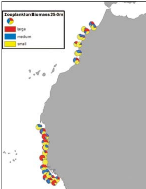
Figure 8a and b: Zooplankton biomass recorded at different depths in the CCLME ecosystem surveys and classified by size of organism
